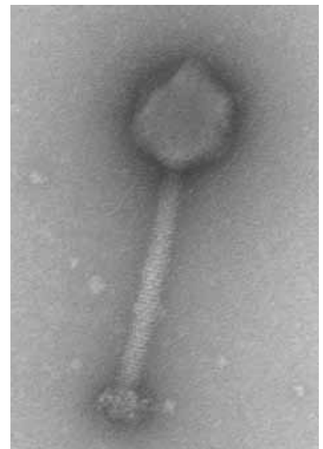
Electron micrograph of a Sb-1-like new potential therapy phage
